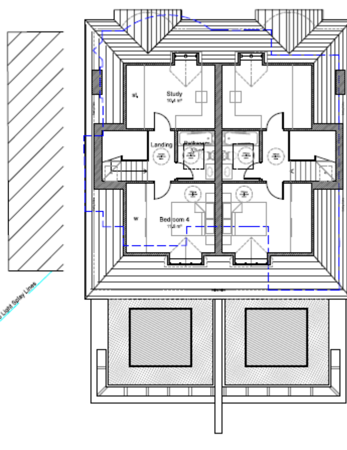
Second Floor Plan - Area 35m sq.
