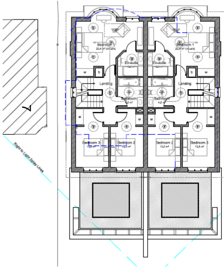
First Floor Plan - Area 66m sq. (01N)
